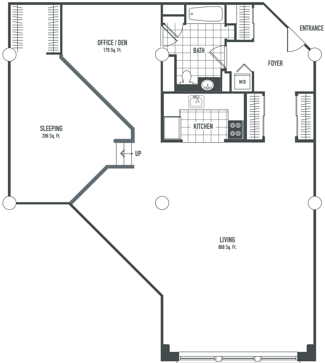
ONE BEDROOM UNIT - TYPE Q 1,523 Sq. Ft.
